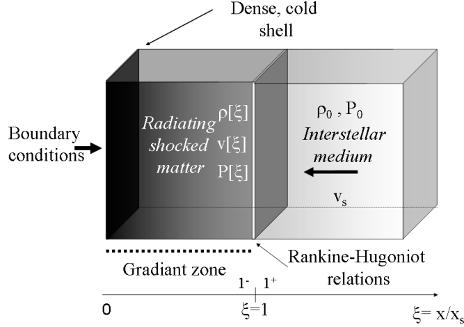
Fig. 1. Schematic representation of radiating shock with the definition of the different physical quantities and notations.
