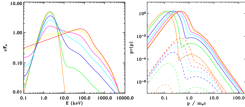
Fig. 1. Photon (left panel) and particle (right panel) distributions in steady state. The total energy is L = 5.5 \times 10^{37} erg s ^{-1} and the fraction of energy injected as soft photons is 0, 10, 30, 50, 70, 90, and 99% for the red, yellow, pink, cyan, blue, green, and orange curves respectively. Dashed lines show the positron distribution. The system is characterized by its size: R = 5 \times 10^7 cm, its optical depths \tau = 2 , and the magnetic field strength B = 2.5 \times 10^6 Gauss. The temperature of the injected soft photons is k_B T = 420 eV and accelerated particles are injected with a power law distribution of slope \Gamma_{inj} = 3 between \gamma_{min} = 1 and \gamma_{max} = 10^3 .
