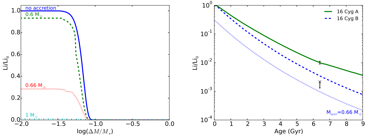
Fig. 1. Left: Lithium abundance profiles just after the accretion of different masses at the beginning of the MS for 16 Cygni B models. Right: Time variations of the lithium surface abundances. The black crosses are the observed lithium abundances (King et al. 1997). The solid and dashed lines represent respectively the models computed for 16 Cyg A and B without any accretion whereas the dotted line corresponds to the models of 16 Cyg B computed with an accreted mass of 0.66 M_{\oplus} .
