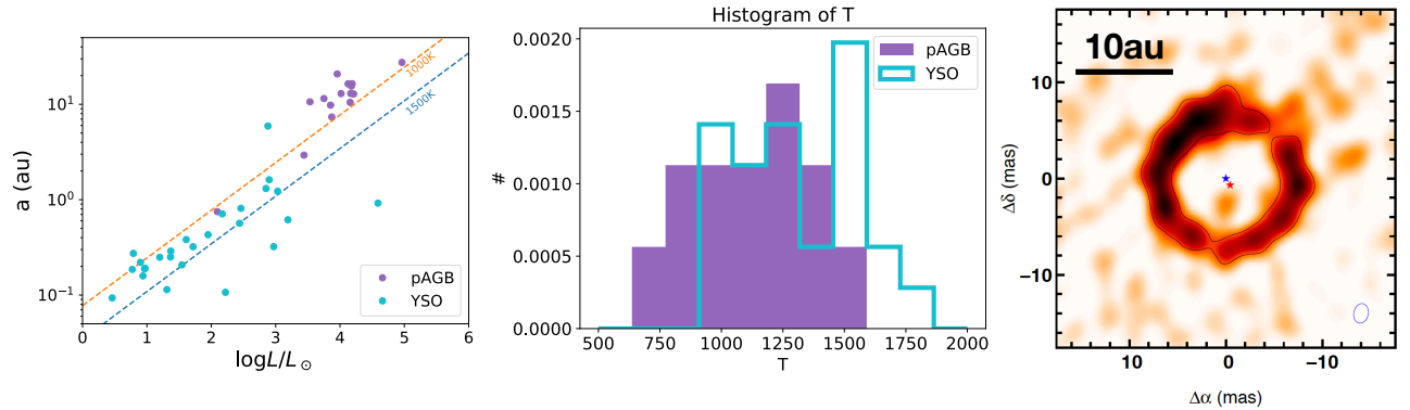
Fig. 1. Left: Near-infrared circumstellar size versus the stellar luminosity for both YSOs and pAGB binaries. The pAGB circumbinary scales with stellar luminosity but the relation is shifted towards larger sizes. Center: Histogram of temperatures for the circumstellar (or circumbinary for pAGBs) environments as measured from VLTI/PIONIER data. The environment of pAGB binaries appear to be colder. Right: The image reconstruction of the circumbinary environment of IRAS08544-4431 as reconstructed with the SPARCO approach (here the central binary was modelled as two point sources and do not appear in the image reconstruction).
