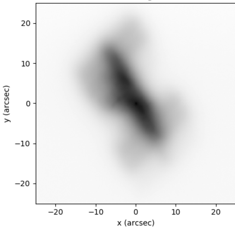
Shift and Add Image of the ISS
