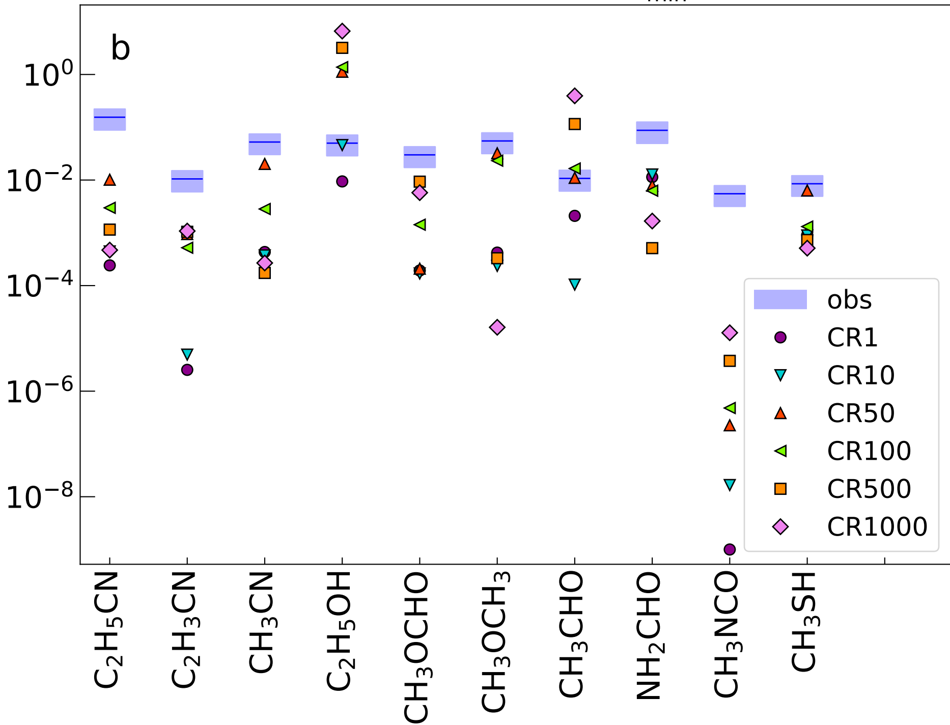
Model results for N2 with T_{\min} = 15 K
