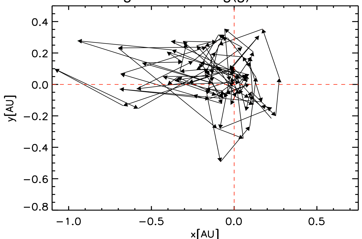
st26gm07n002 - \log(g) = -0.85
