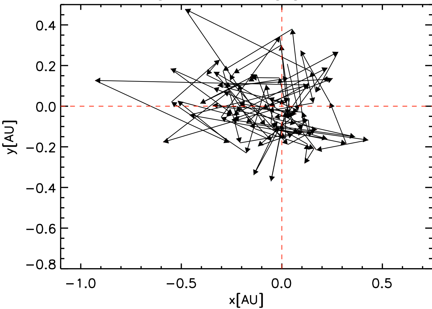
st28gm06n26 - \log(g) = -0.70
