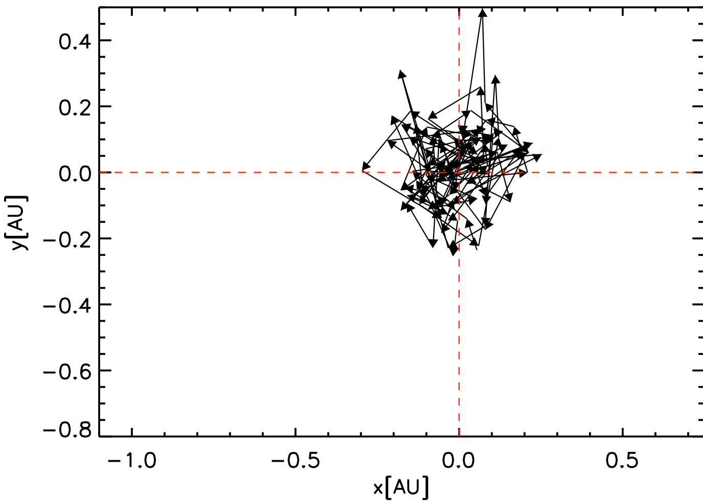
st28gm06n26 - \log(g) = -0.70
