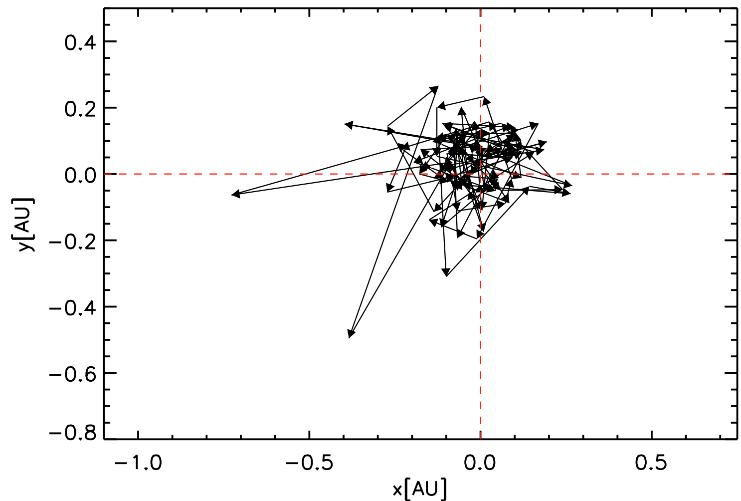
st26gm07n002 - \log(g) = -0.85
