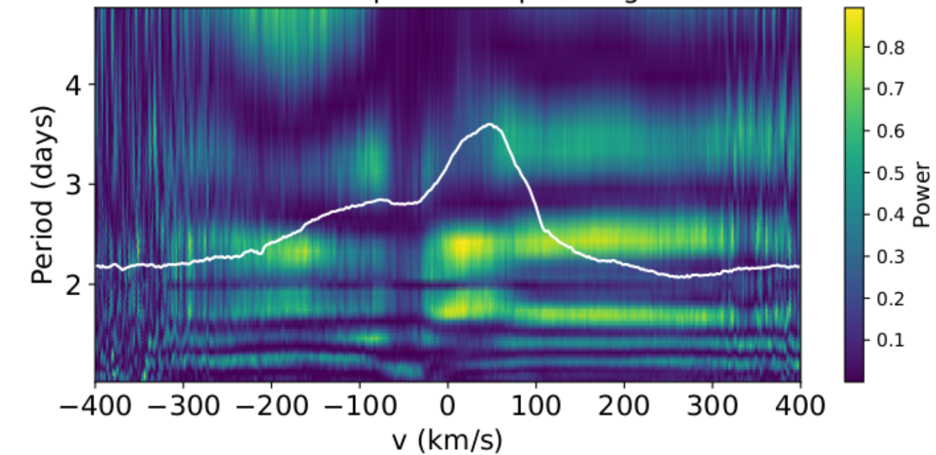
Residual Ha profile 2D-periodogram
