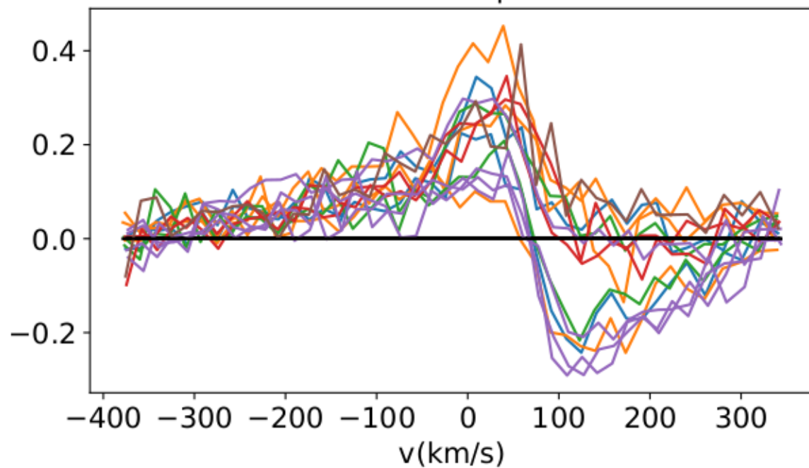
Residual Hb profile
