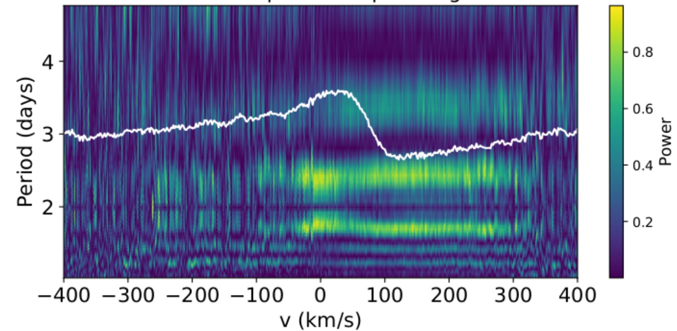
Residual Hb profile 2D-periodogram
