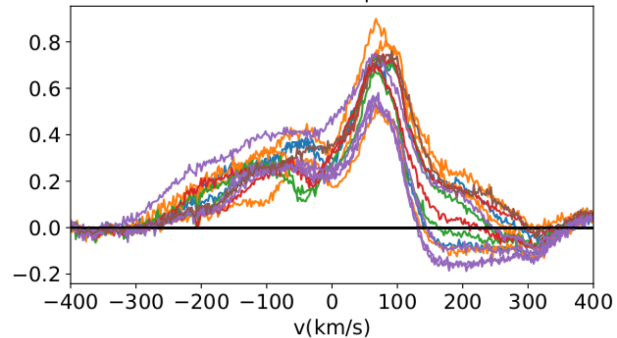
Residual Ha profile
