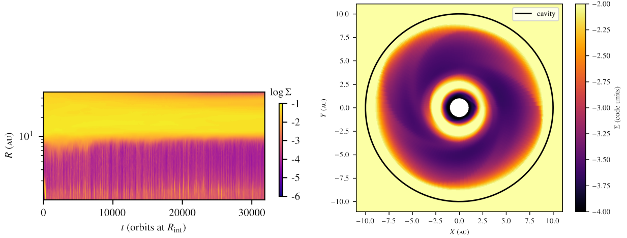
Fig. 1. Left: Spatio-temporal diagram of the surface density for the fiducial 2.5 D simulation. Right: Surface density in the midplane and at a given time for the fiducial 3 D simulation. The black circle indicates the location of the outer edge of the cavity.
