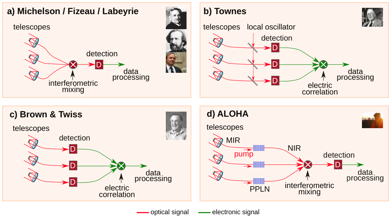
Fig. 1. Comparative presentation of the three classic configurations and the ALOHA concept (bottom right). Top left: the most common method uses the field correlation. The two intensity correlation measurements (direct and heterodyne) are shown top right and bottom left).
