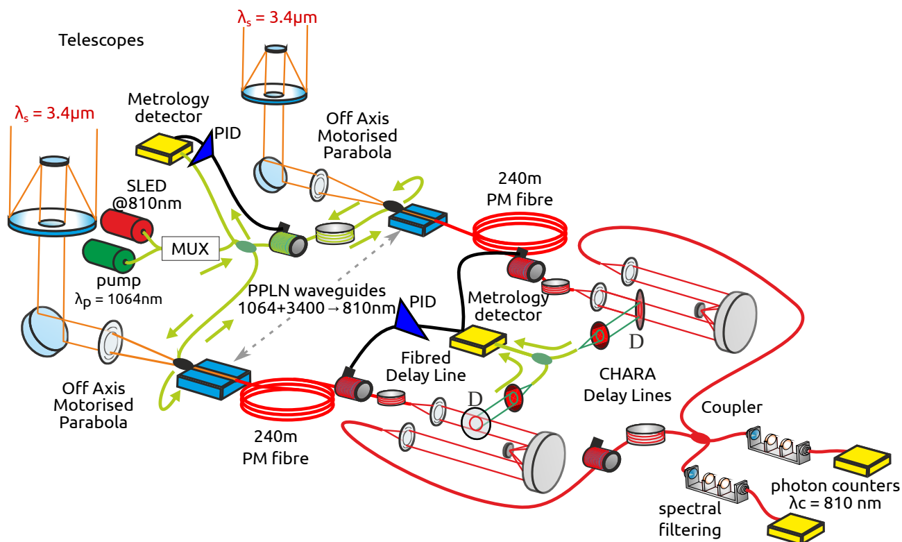
Fig. 2. ALOHA implementation at CHARA: the light collected at 3.4 \mu\text{m} is converted at 810 nm thanks to a 1064 nm pump laser and nonlinear PPLN waveguides. The pump light propagates through 50 m long PM fibres. The converted light then passes into 240 m PM fibres towards the CHARA free space delay lines. After interferometric recombination, the interferometric signal is detected in the photon counting regime. Two cascaded servo control systems are used to stabilise the OPD of the pump and converted signal fibres. SLED: Superluminescent Diode, PID: Proportional-Integral-Derivative controller, MUX: Multiplexer.
