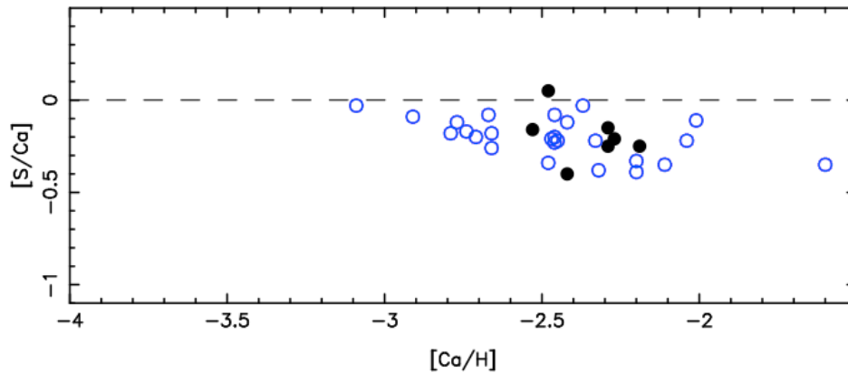
Fig. 3. [\text{S}/\text{Ca}] vs. [\text{Ca}/\text{H}] . Symbols like in Fig. 2.
