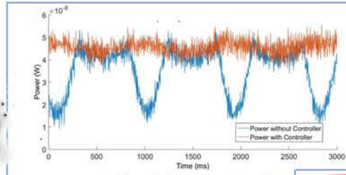
Coupled power over time
