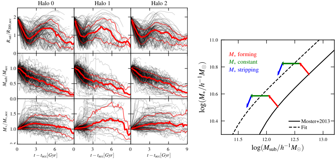
Fig. 3. Left: time evolution of subhalo/satellite galaxy properties since accretion: cluster-centric distance, subhalo mass and stellar mass, from top to bottom. The masses are normalized by their values at the time of accretion. Right: summary of the SHMR evolution for satellite galaxies. Three phases can be identified in the process: dark matter stripping + star-formation (red arrows), dark matter stripping at constant stellar mass (green arrows) and dark + stellar matter stripping (blue arrows).
