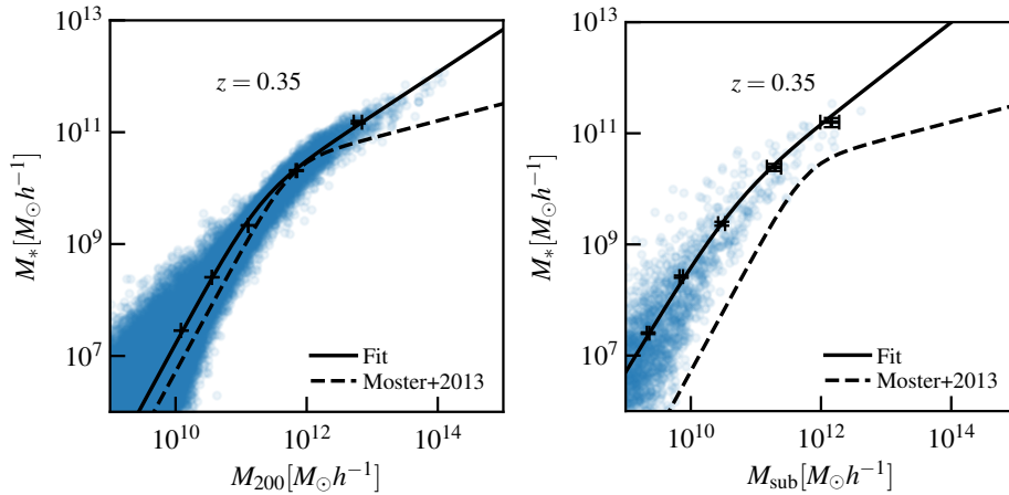
Fig. 2. Left: SHMR for central galaxies at z = 0.35 . Right: SHMR for the satellite galaxies of the 3 cluster-like haloes at z = 0.35 . The solid black line shows the best-fit relation and the dashed line shows the relation from Moster et al. (2013) as reference. Both figures are adapted from Paper II.
